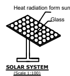
SOLAR SYSTEM
