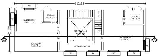
PRO.FIRST FLOOR PLAN
