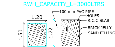
PLAN & SECTION OF RAIN WATER COLLECTION TANK
