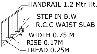
STAIR DETAIL
