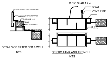
RAIN WATER HARVESTING NTS
