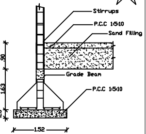
COLUMN DETAIL
