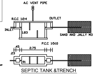
SEPTIC TANK & TRENCH
