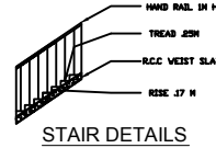
STAIR DETAILS
