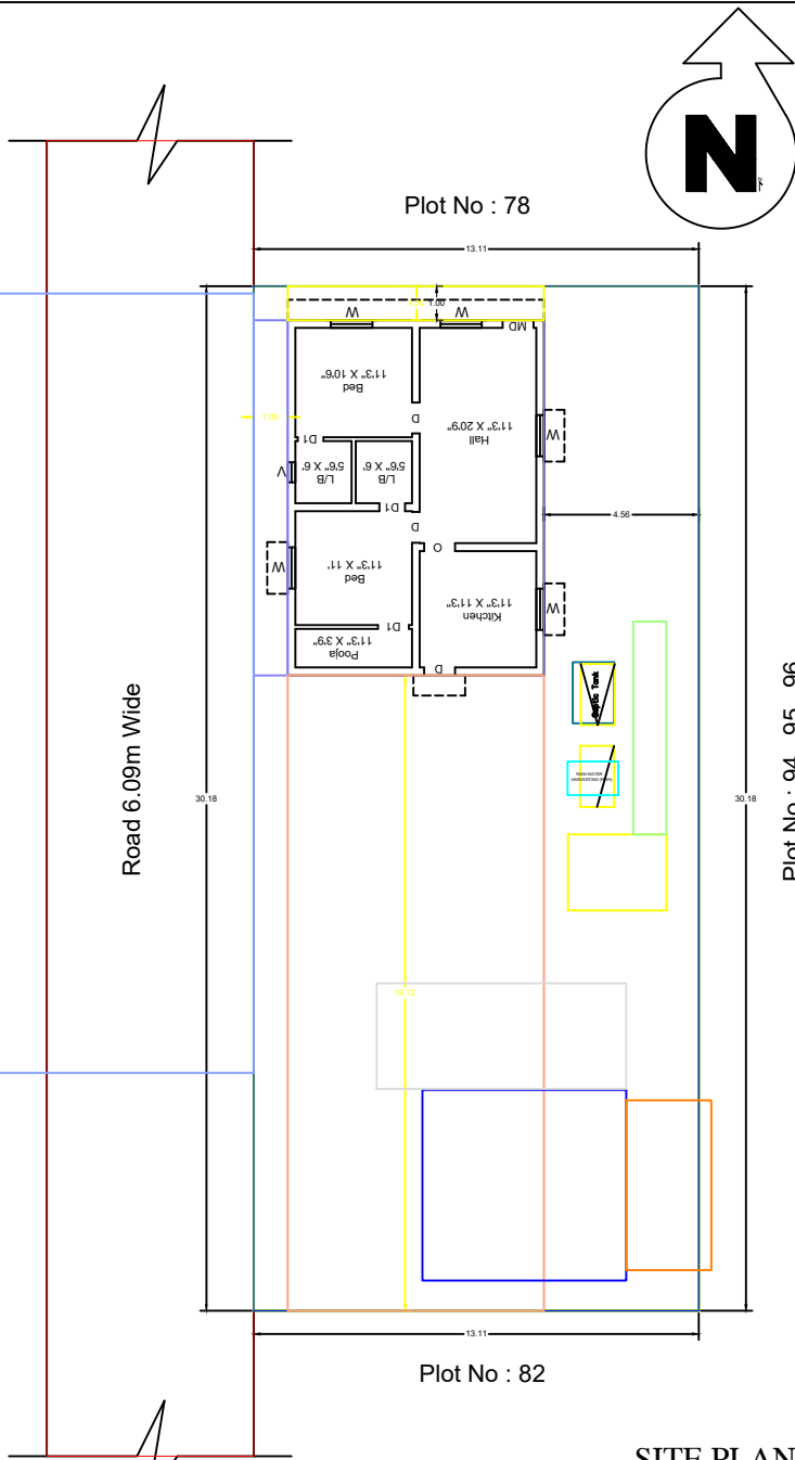
SITE PLAN
