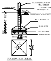
FOUNDATION DETAIL
