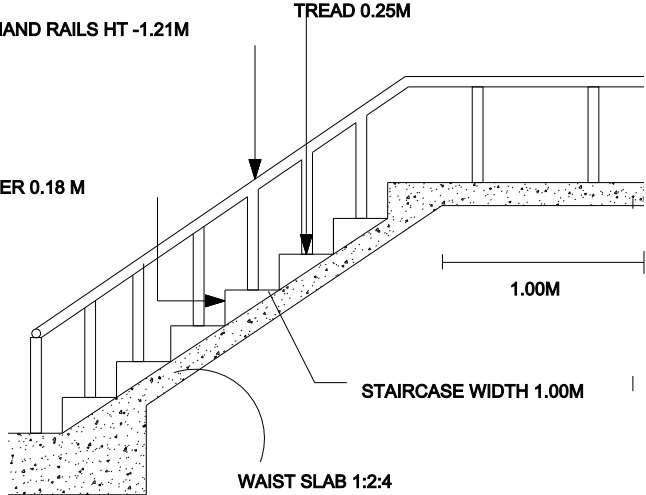
STAIRCASE DETAILS
