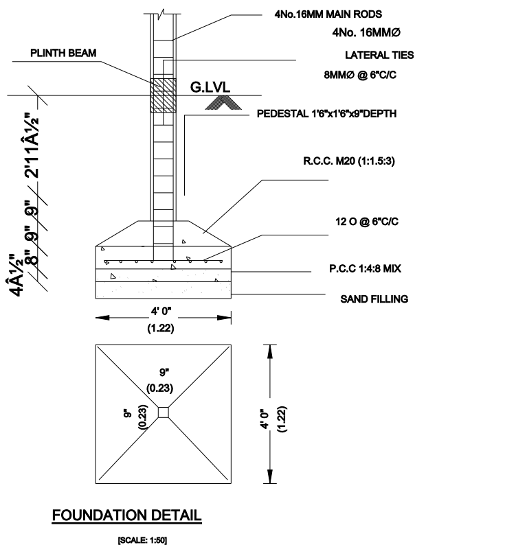
FOUNDATION DETAIL
