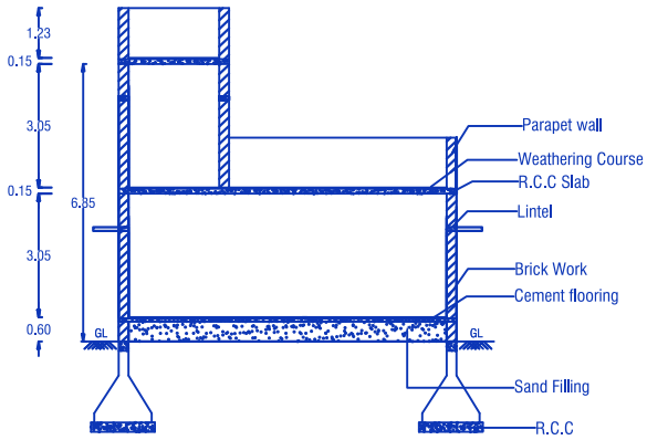
CROSS SECTION ON 'AB'
