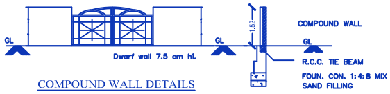
COMPOUND WALL DETAILS
