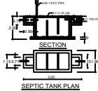
SEPTIC TANK PLAN
