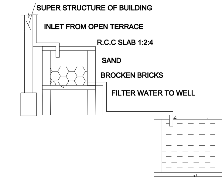
Rainwater harvesting
