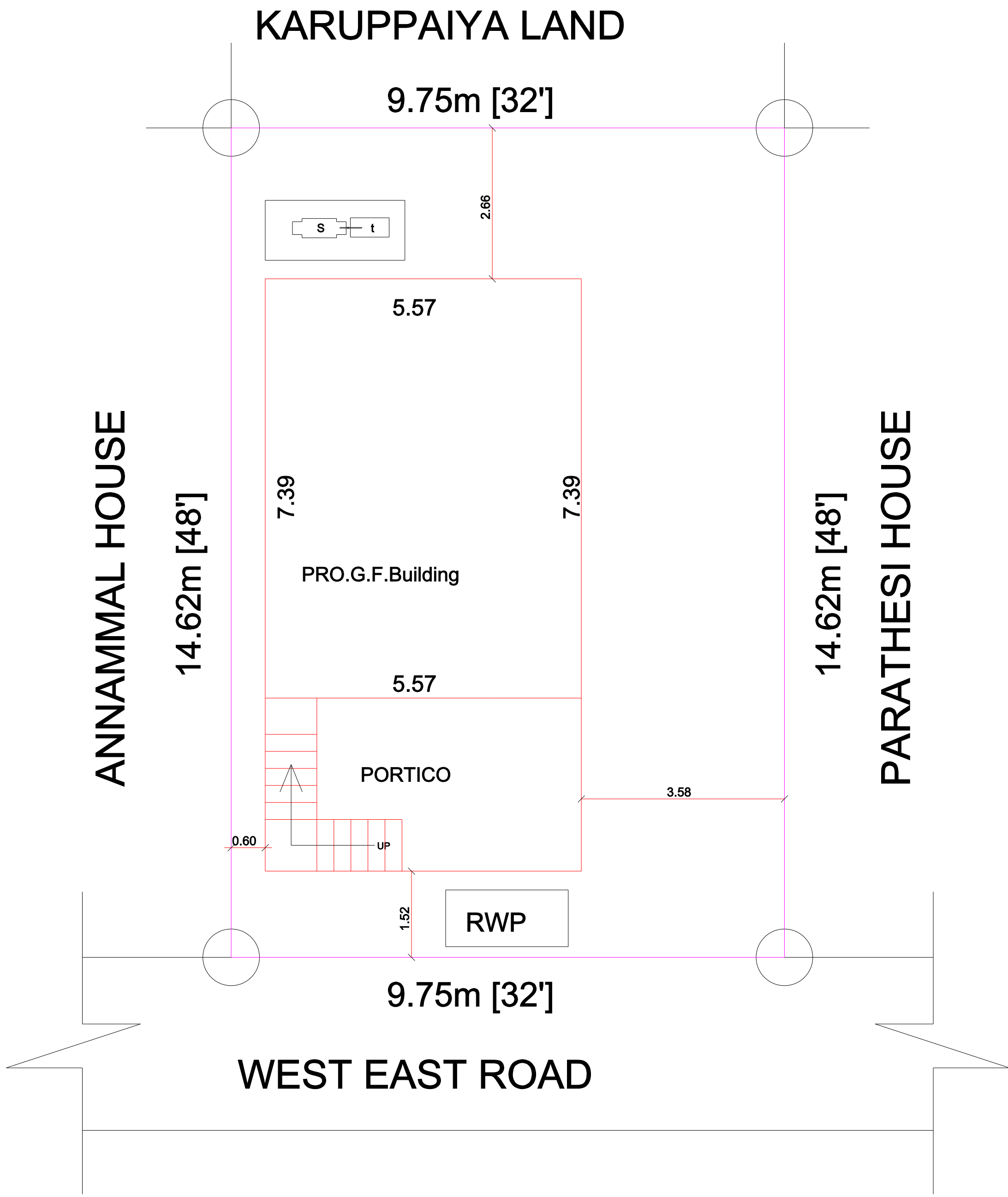
SITE PLAN
