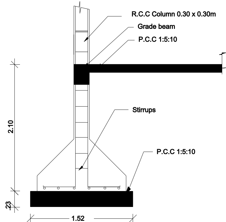
Column Detail
