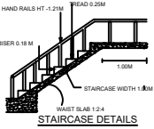
STAIRCASE DETAILS
