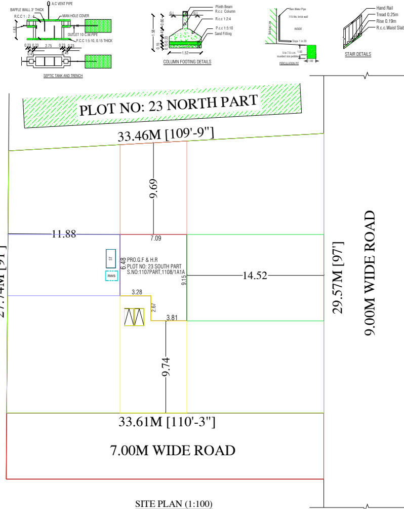
SITE PLAN (1:100)
