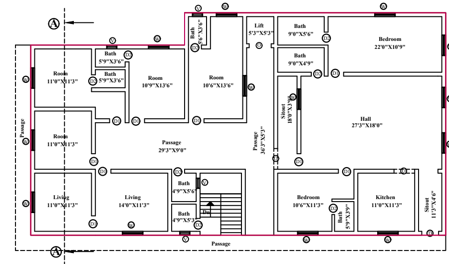
EXG.FIRST FLOOR PLAN
