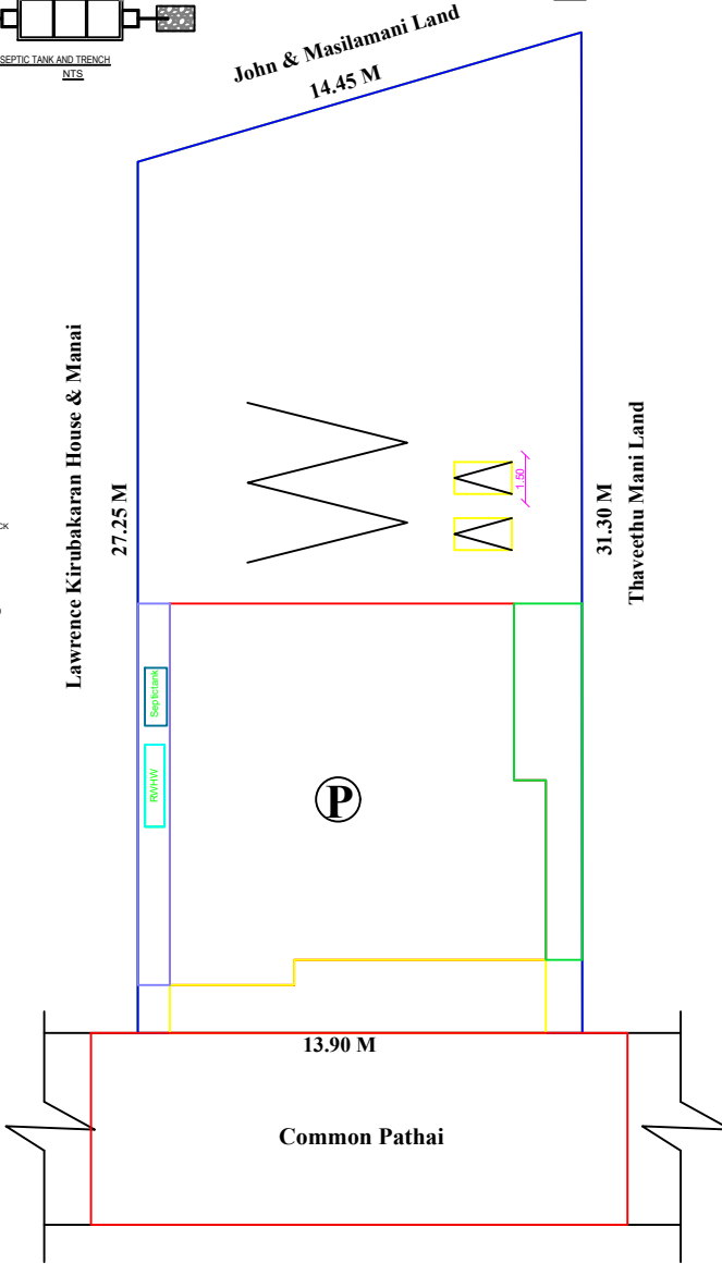
SITE PLAN
