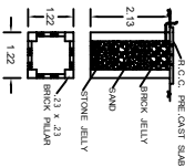
PLAN & SECTION OF RAIN WATER COLLECTION WELL
