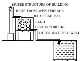
Rainwater harvesting
