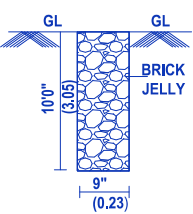
PERCULATION PIT
