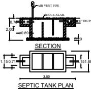
SEPTIC TANK PLAN
