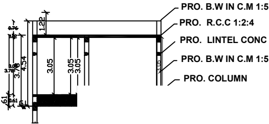
SECTION
