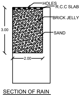
SECTION OF RAIN
