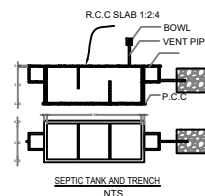
SEPTIC TANK AND TRENCH NTS
