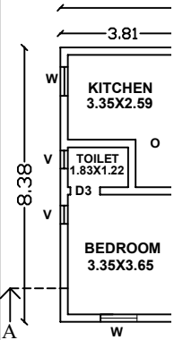
PROPOSED GROUND FLOOR PLAN
