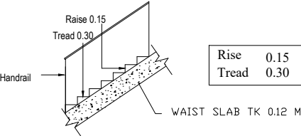
STAIRCASE DETAIL
