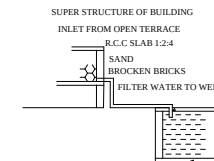
Rainwater harvesting
