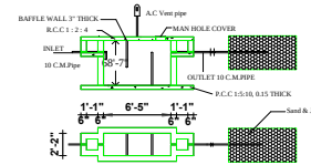
Septic tank and trench
