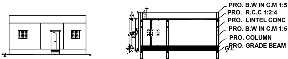
SECTION ON A A
