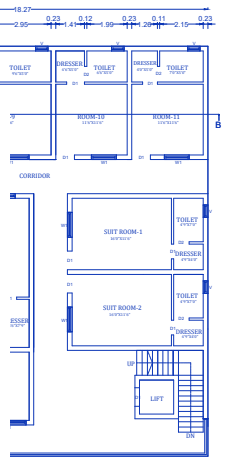
1 ST FLOOR PLAN
