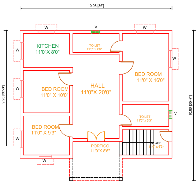
G.F. PLAN
