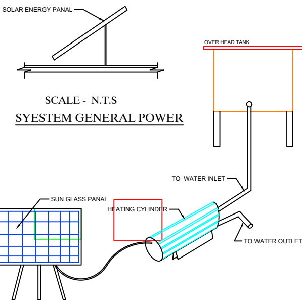
SOLAR WATER HEATING SYSTEM SCALE - N.T.S
