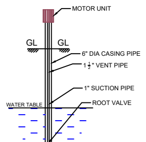
SEC.OF BOREWELL
