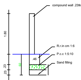
Compound Wall Detail SCALE : (1:50)
