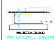
RWH_SECTION (SAMPLE) RWH_CAPACITY_L = 2000LTRS
