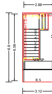
S.FLOOR PLAN
