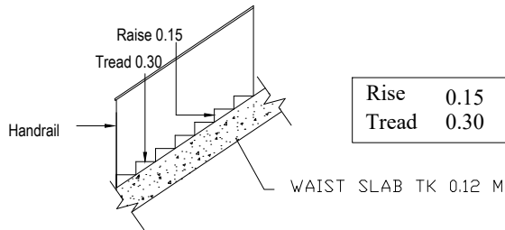
STAIRCASE DETAIL
