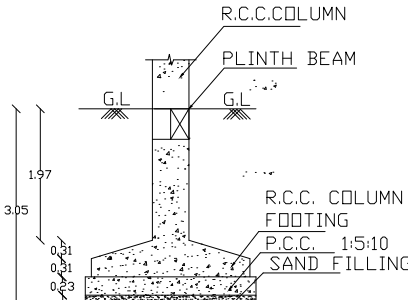
FOUNDATION DETAIL
