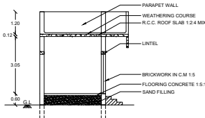
SECTION ON 'A-A'
