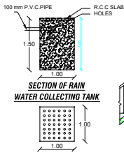
SECTION OF RAIN WATER COLLECTING TANK
