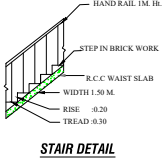
STAIR DETAIL
