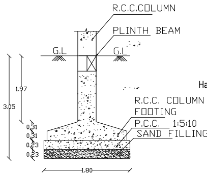
FOUNDATION DETAIL
