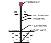
SEC.OF BOREWELL
