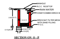
SECTION ON O - P
