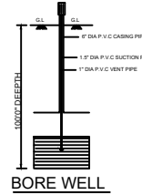
BORE WELL
