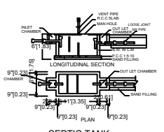
SEPTIC TANK
