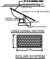
SOLAR SYSTEM
