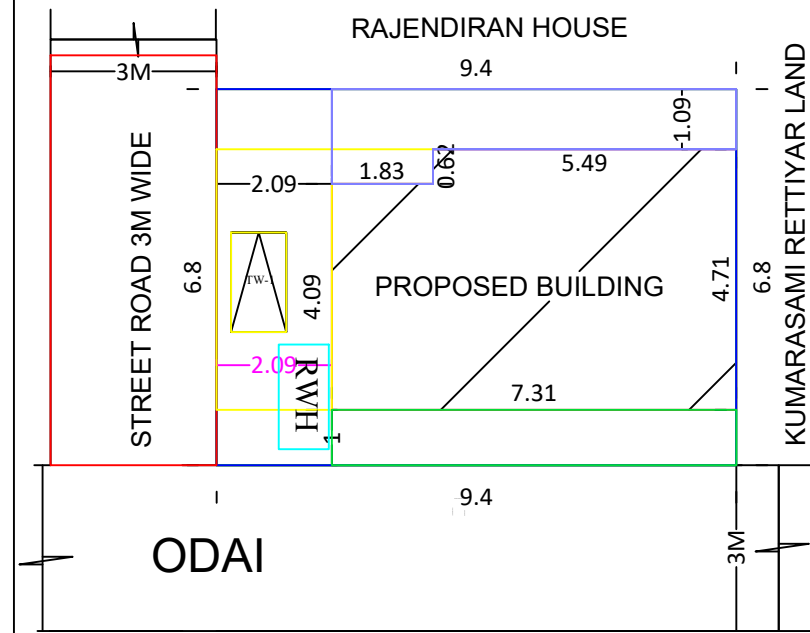
SITE PLAN 1:500 SCALE
