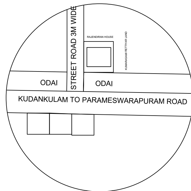
KEY PLAN 1:1000 SCALE
