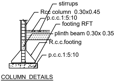
COLUMN DETAILS
