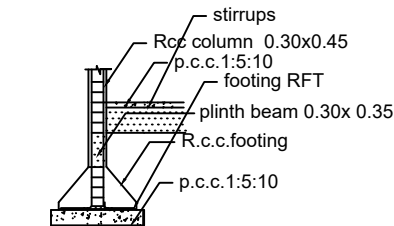
COLUMN DETAILS
