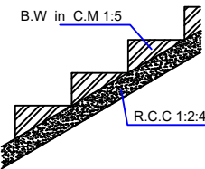
STAIRCASE
