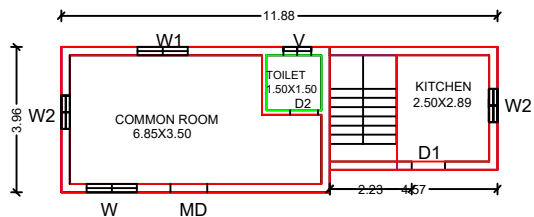
GROUND FLOOR
