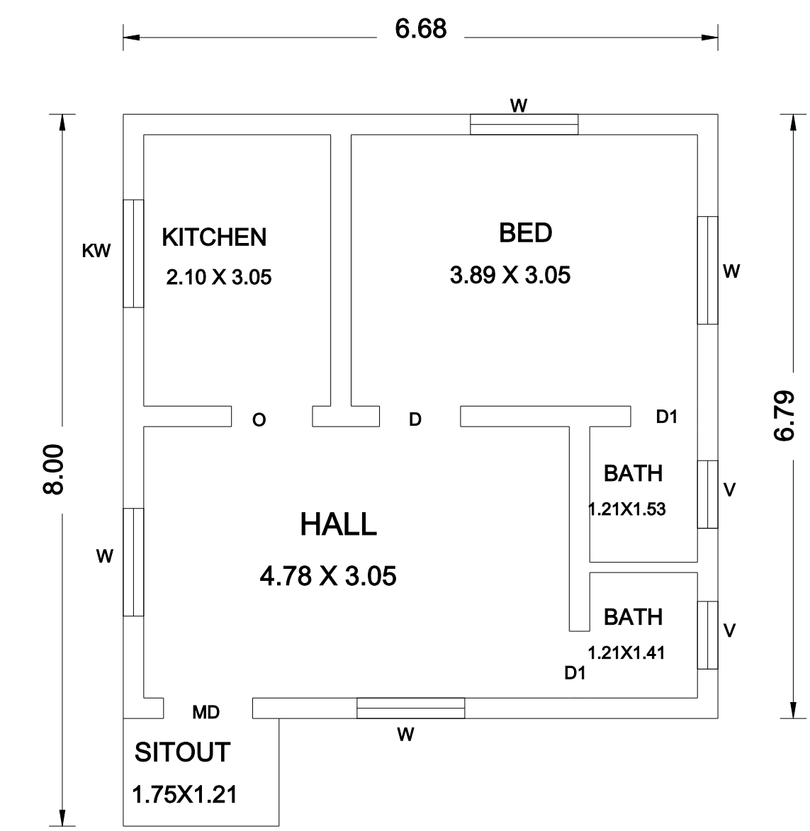
PRO.G.FLOOR PLAN
