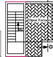
SECOND FLOOR PLAN (HEADROOM)
