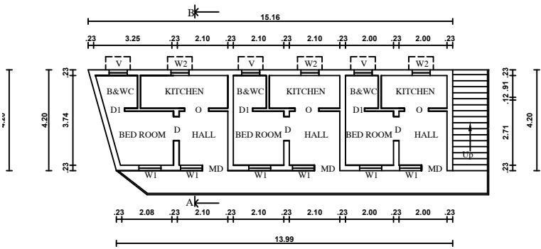
PRO FIRST FLOOR PLAN SCALE-1:100
