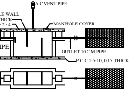
SEPTIC TANK & TRENCH
