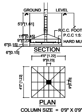
FOUNDATION DETAILS
