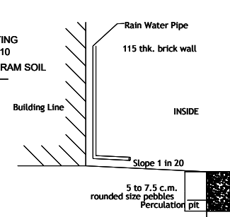
PERCOLATION PIT
