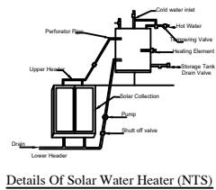
Details Of Solar Water Heater (NTS)
