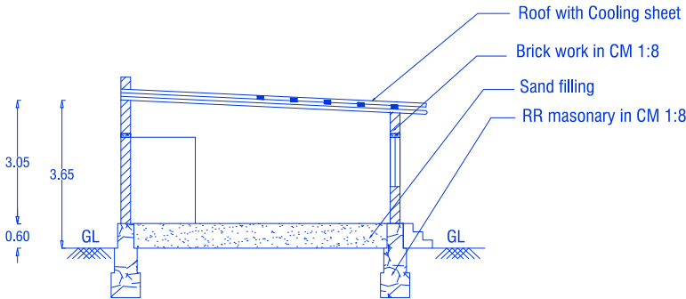
CROSS SECTION ON 'AB'
