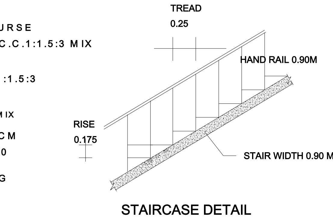
STAIRCASE DETAIL
