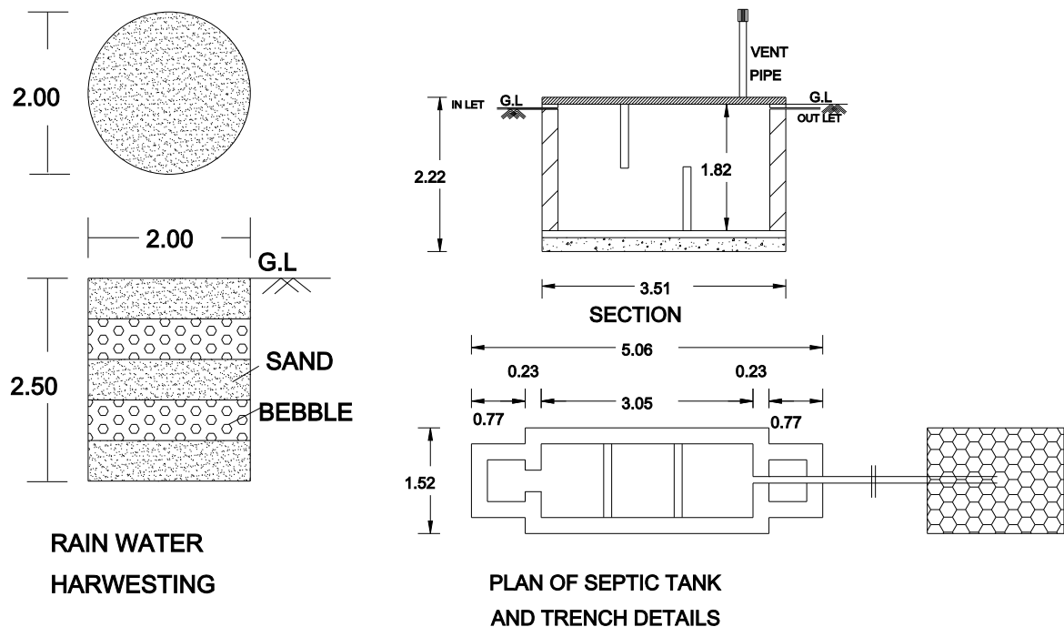
PLAN OF SEPTIC TANK AND TRENCH DETAILS
