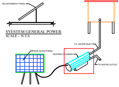
SOLAR WATER HEATING SYSTEM SCALE - N.T.S.
