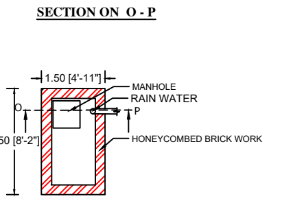
PLAN RAIN WATER HARVESTING
