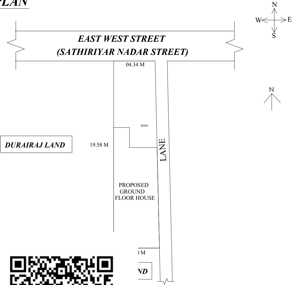
SITE PLAN
