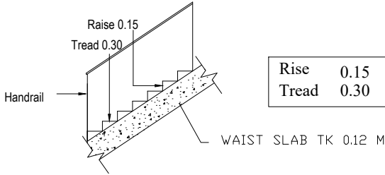
STAIRCASE DETAIL
