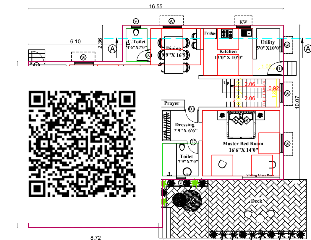
PRO.GROUND FLOOR PLAN
