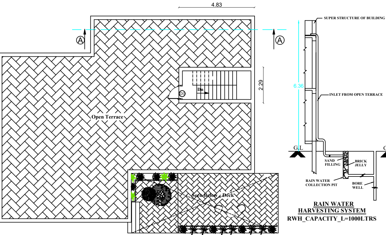
PRO.TERRACE FLOOR PLAN(HEADROOM)
