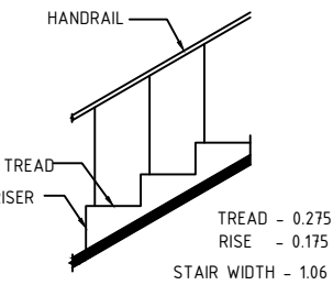
STAIRCASE DETAILS
