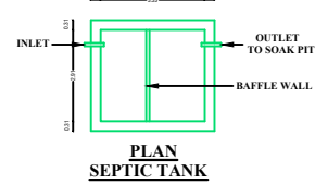
PLAN SEPTIC TANK
