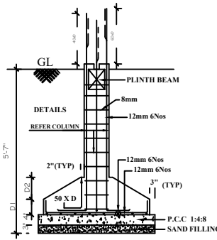
FOUNDATION DETAILS
