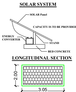
SOLAR SYSTEM
