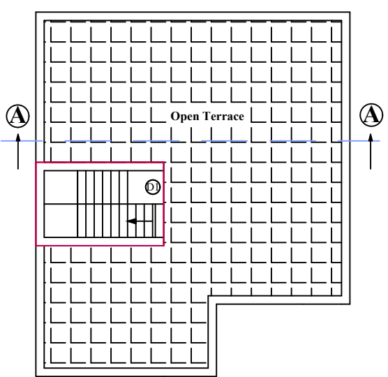
TERRACE FLOOR PLAN(HEADROOM)
